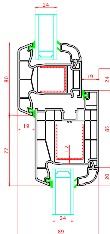
C-C' SECTION
