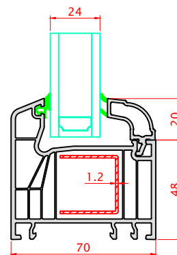
D-D' SECTION
