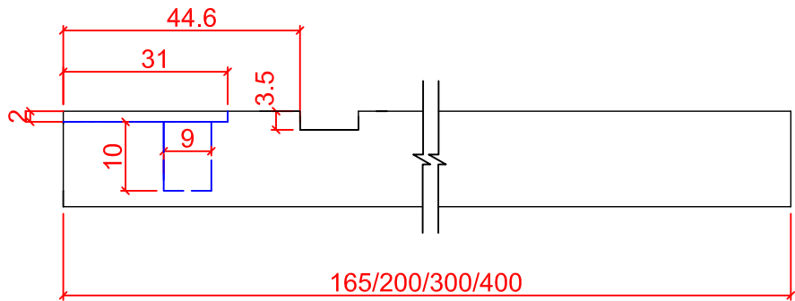
DETAIL B
