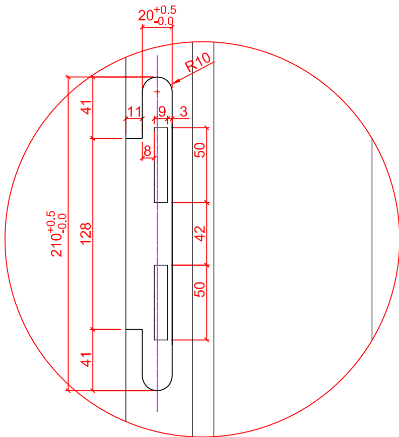
DETAIL A
